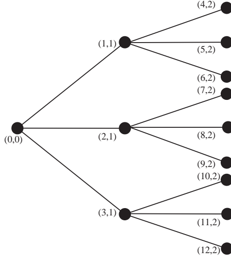
Figure 2: Scenario Tree: Example
