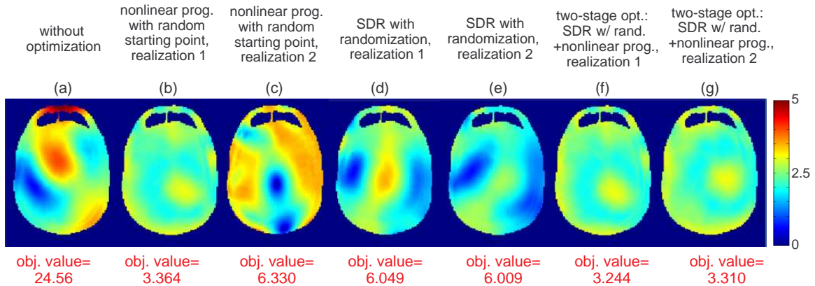
Fig. 9. B_1 maps of various optimization methods.
