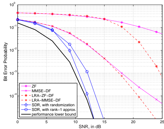
Fig. 3. Bit error probability performance of various MIMO detectors in a QPSK 40 \times 40 MIMO system. ‘ZF’— zero forcing, ‘MMSE’— minimum mean square error, ‘DF’— decision feedback, ‘LRA’— lattice reduction aided. ‘performance lower bound’ is the bit error probability when no MIMO interference exists.
