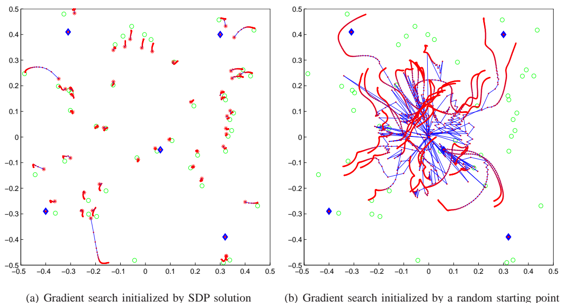
Fig. 10. Refinement through a gradient search method for a 50 node network
