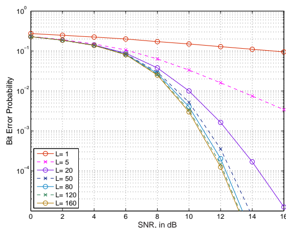
Fig. 5. Performance of various numbers of randomizations in MIMO detection, under the same simulation settings as that in Fig. 3.
