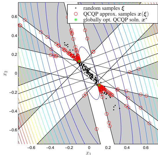
Fig. 6. Illustration of randomizations in \mathbb{R}^2 , for Problem (16). The gray area is the feasible set and colored lines the contour of the objective.
