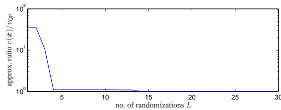
Fig. 7. A realization of the actual approximation accuracy of SDR for the problem instance in Fig. 6.
