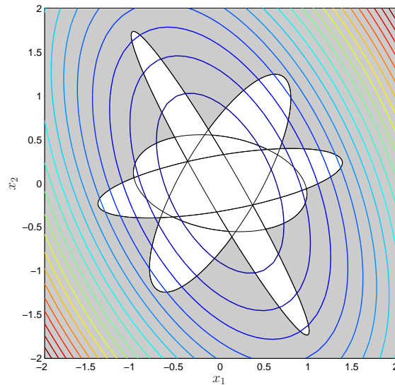
Fig. 1. A nonconvex QCQP in \mathbb{R}^2 . Colored lines: contour of the objective function; gray area: the feasible set; black lines: boundary of each constraint.
