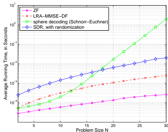
Fig. 4. Complexity comparison of various MIMO detectors. SNR= 12dB.
