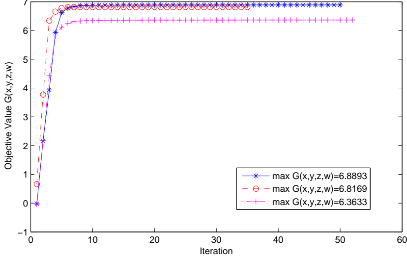
FIG. 5.1. Convergence results of MBI for (E_6)
